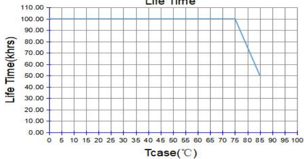
Life Time
