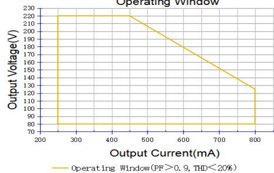
Operating Window
